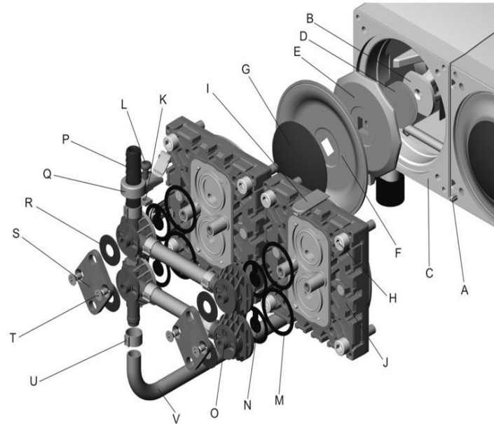
View of the disassembled pump head parts (fig.: MD 4C NT)
